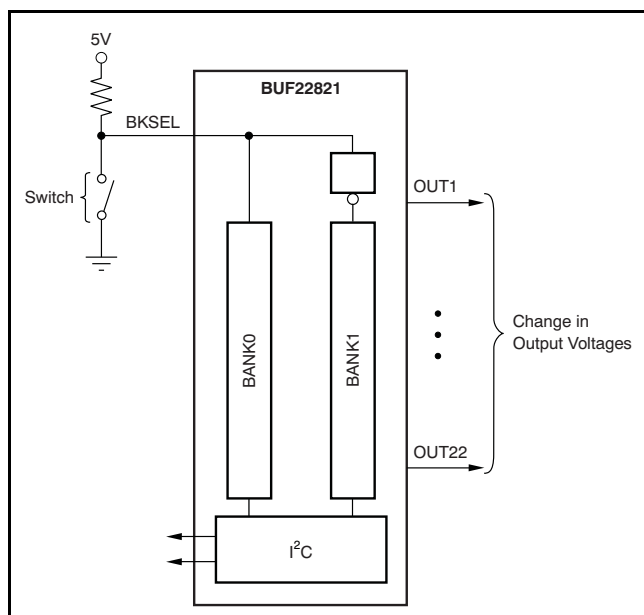
Figure 19. Gamma Control
